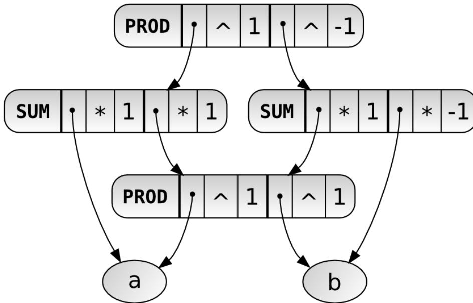
Figure 3.1: expr DAG
