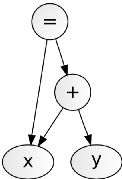
Figure 2.2: Expression DAG
