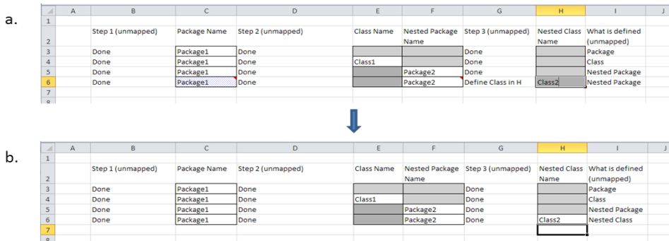
Figure 2.46: Defining Class2 Inside of Package2
