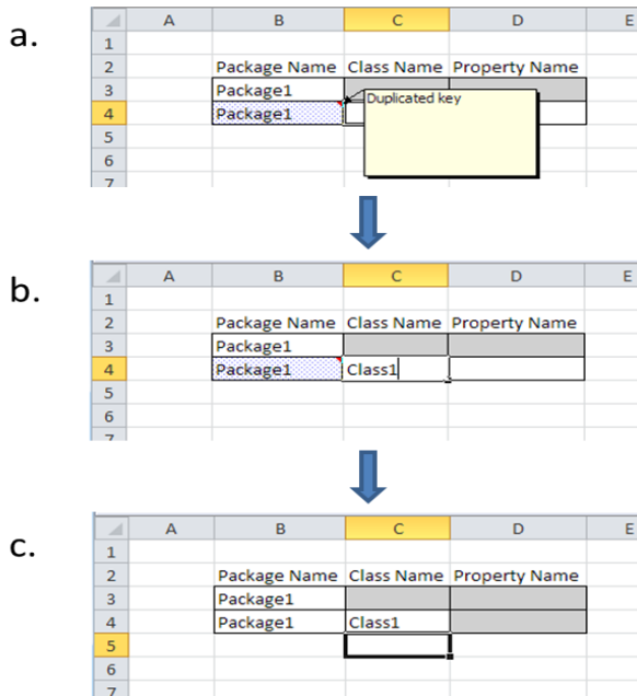
Figure 2.11: Defining Class1
