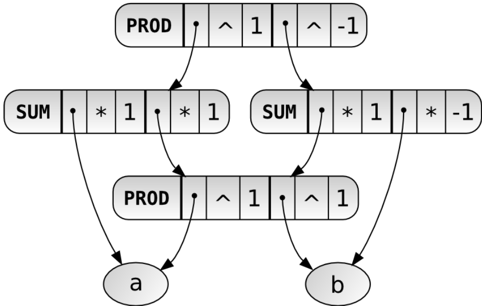
Figure 3.1: expr DAG
