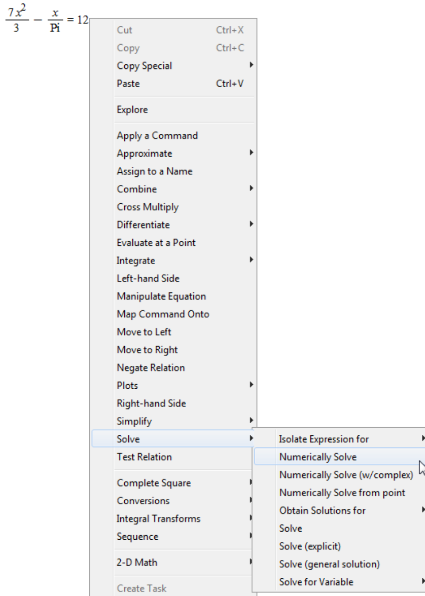
Figure 2.3: Finding the Approximate Solution to an Equation
