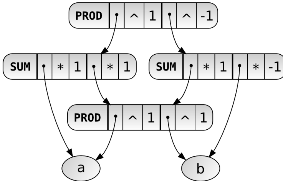
Figure 3.1: expr DAG
