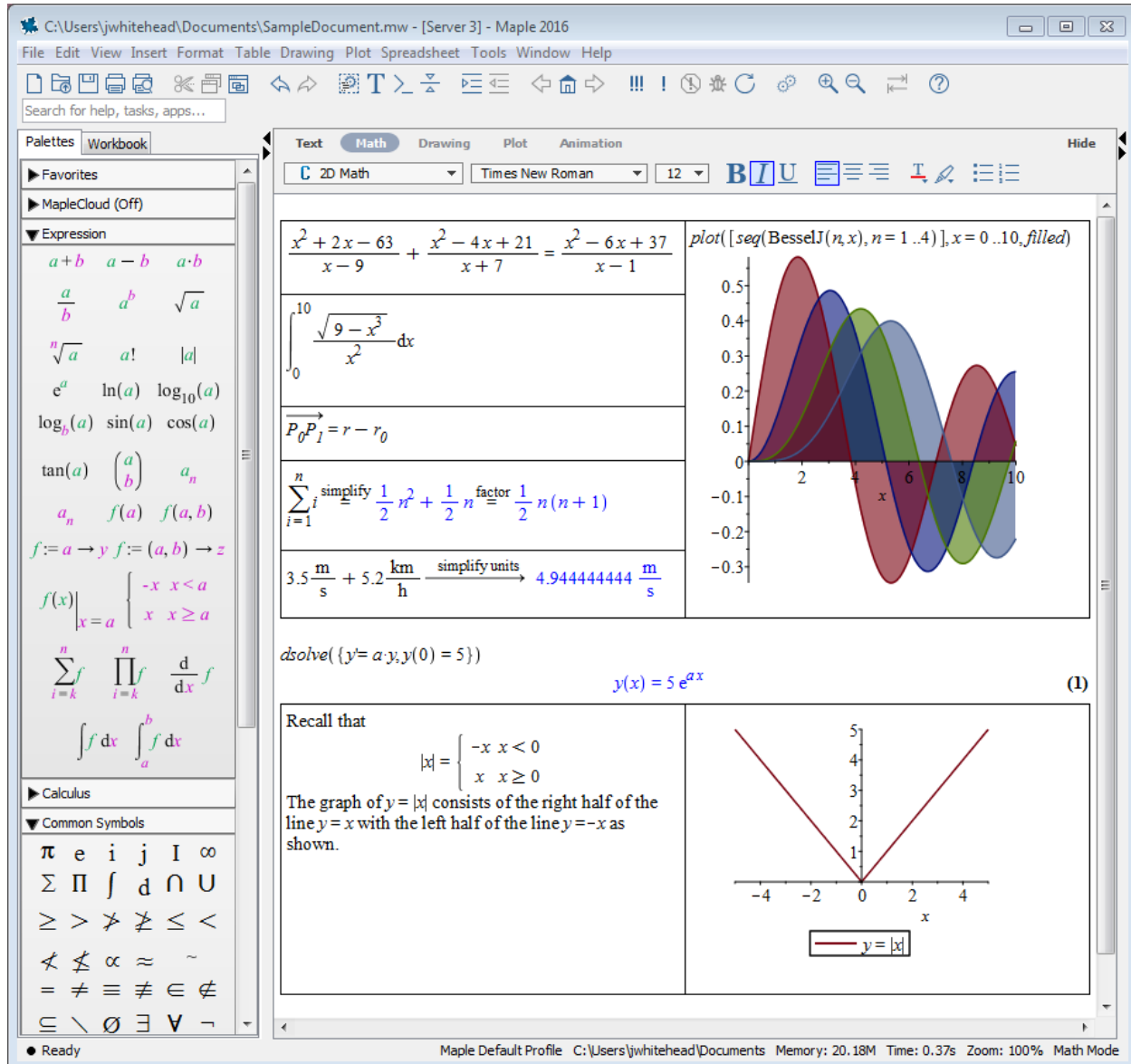
Figure 1.1: The Maple Environment
