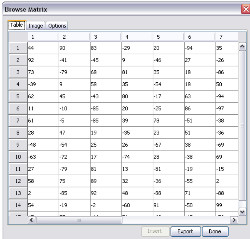
Figure 5.5: Matrix Browser
