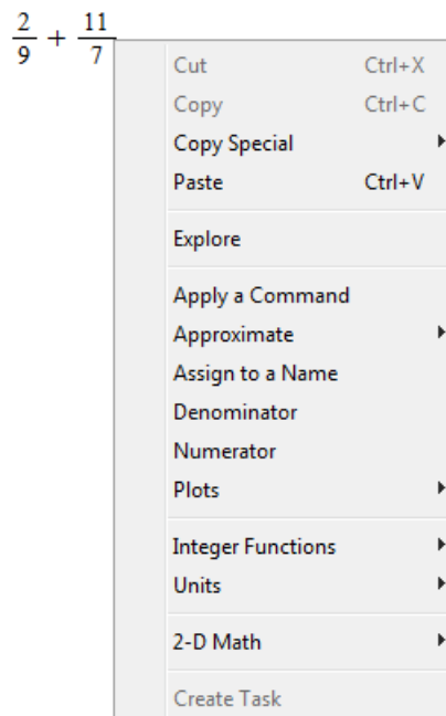
Figure 2.1: Context Menu
