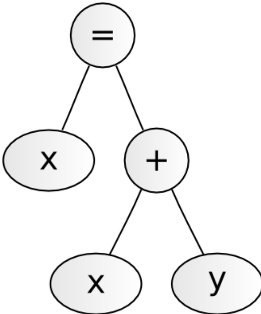
Figure 2.1: Expression Tree
