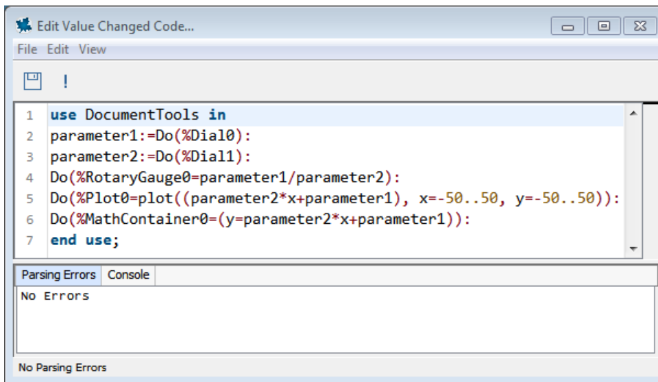
Figure 10.5: DialComponent Action Code Editor
