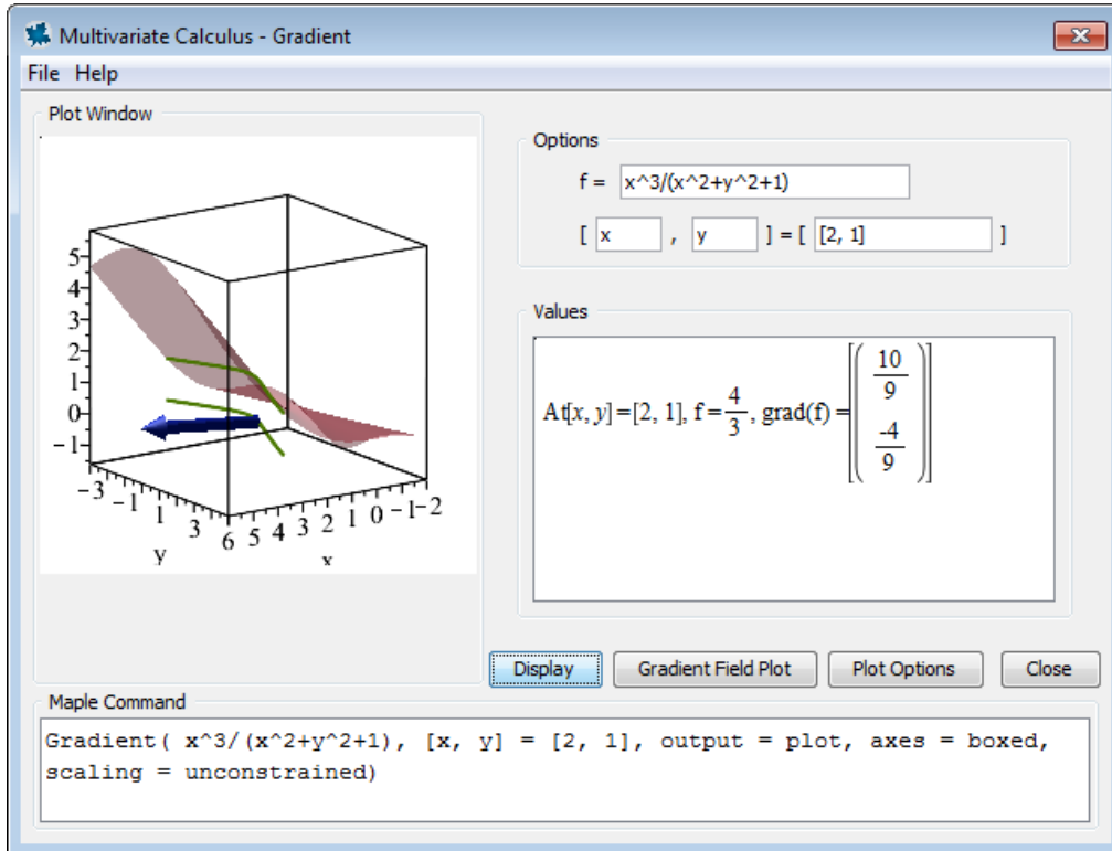
Figure 5.11: Calculus 1 Differentiation Methods Tutor
