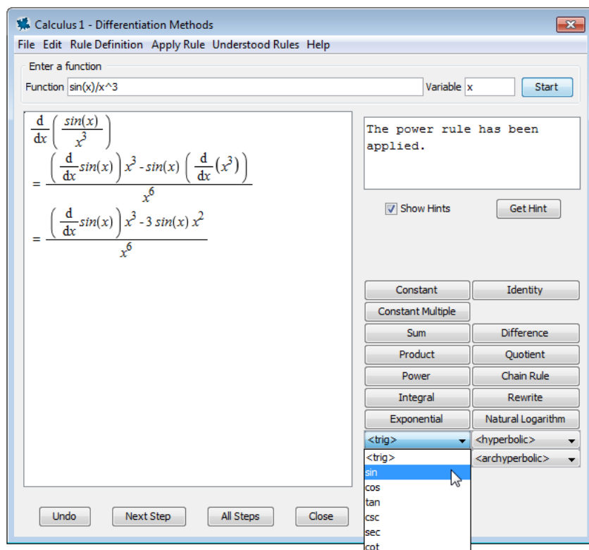
Figure 5.10: Calculus 1 Derivatives Tutor
