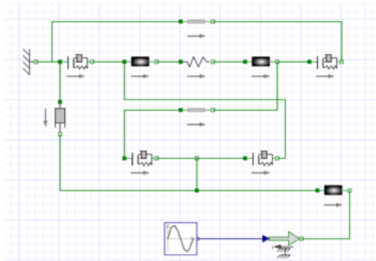
Figure 2.17: Hydraulic Model
