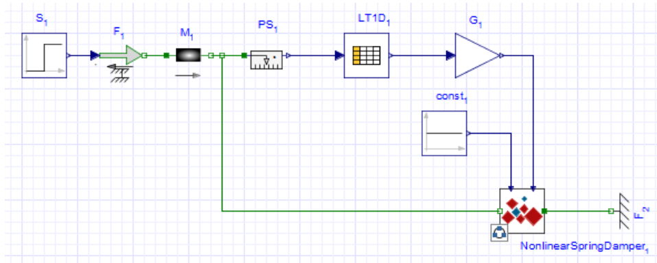
Figure 6.2: Nonlinear Damper Model
