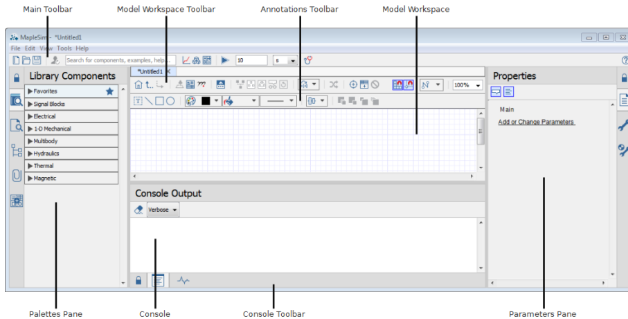
Figure 1.7: MapleSim Window
