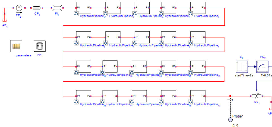
Figure 6.27: Water Hammer
