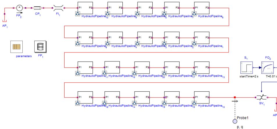
Figure 6.27: Water Hammer
