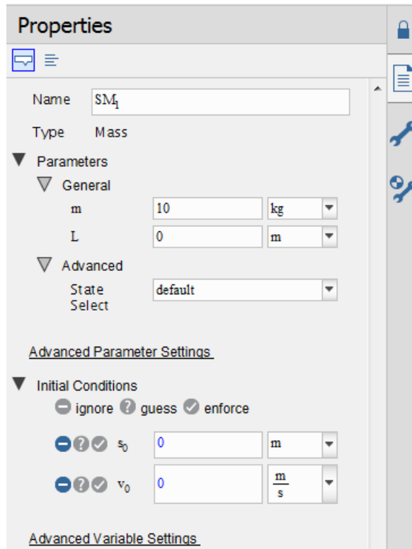
Figure 2.6: Initial Conditions
