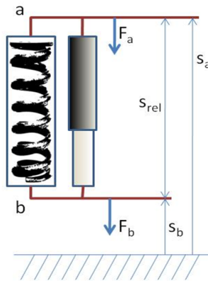
Figure 3.10: Nonlinear Spring-Damper Custom Component
